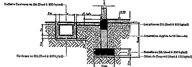
DETAILS B
