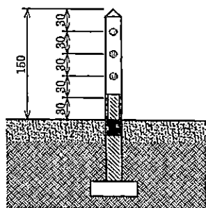
DETAILS A
